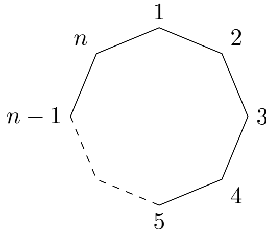
Figure 5.2.1 A regular n -gon
