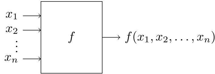
Figure 14.3.8 A switching function of n variables
